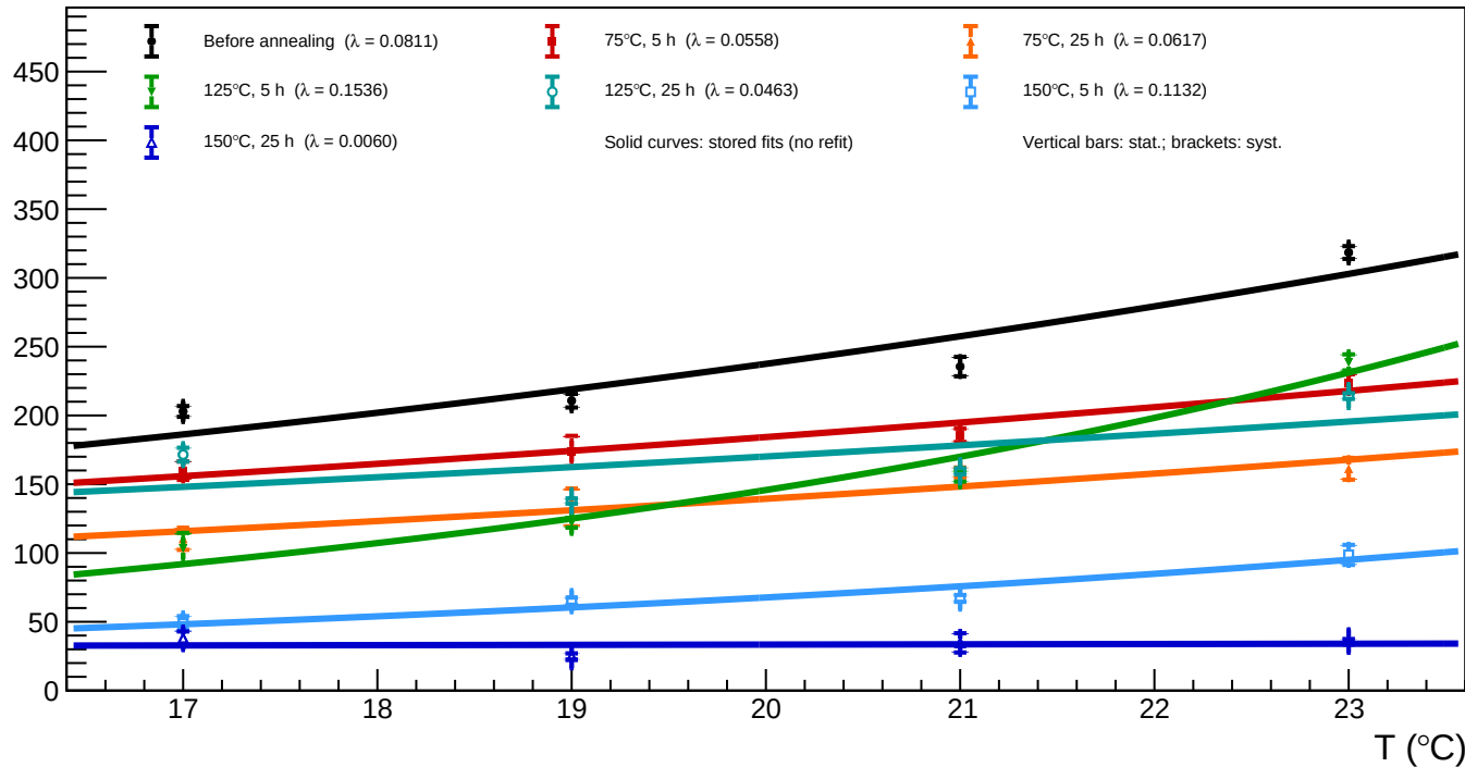
B1_v=3 - Spot 53 (x = 1682.13, y = 919.01): luminosity vs temperature for all annealing phases
