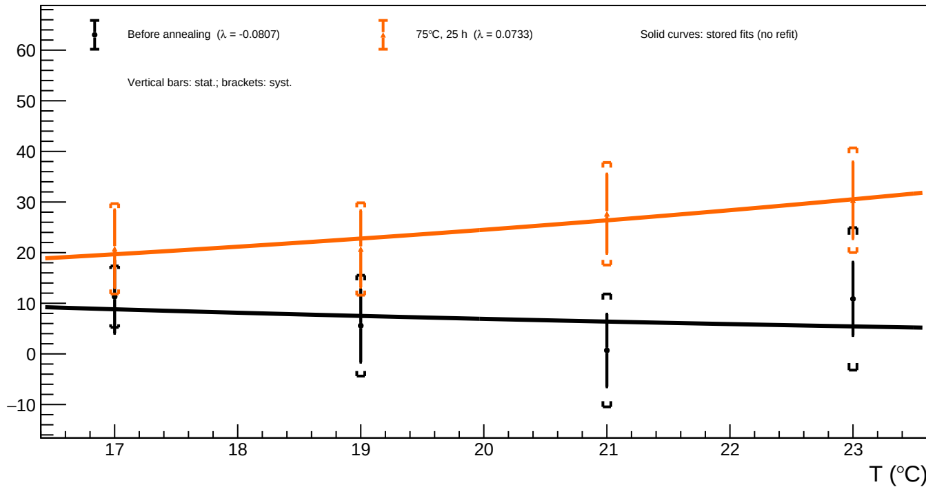
B1_v=3 - Spot 54 (x = 1708.66, y = 451.78): luminosity vs temperature for all annealing phases
