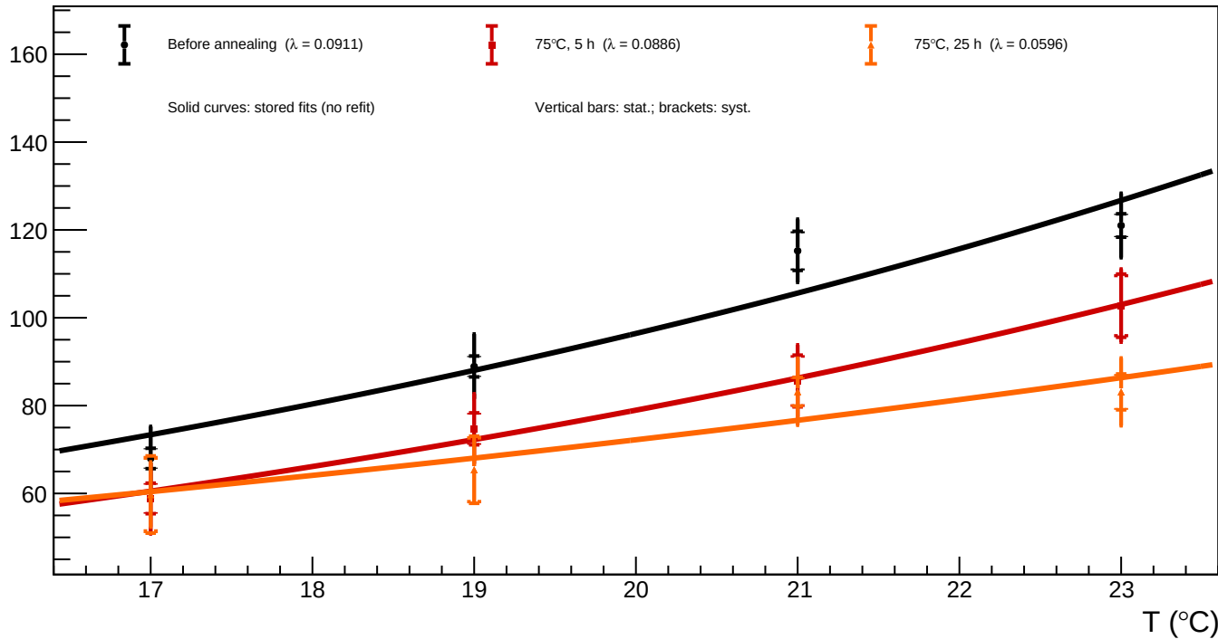
B1_v=3 - Spot 56 ( x = 1754.68 , y = 207.45 ): luminosity vs temperature for all annealing phases
