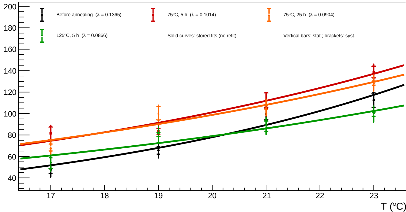
B1_v=3 - Spot 58 ( x = 1814.44 , y = 139.58 ): luminosity vs temperature for all annealing phases
