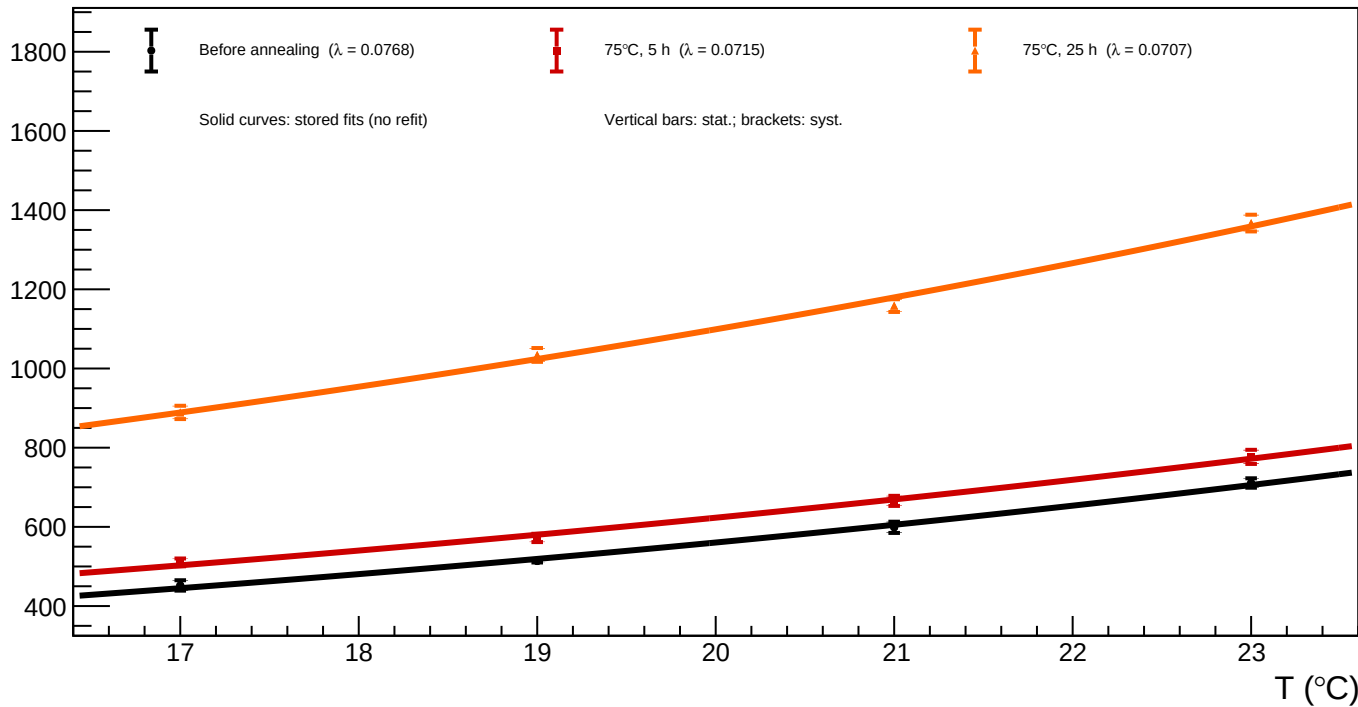
B1_v=3 - Spot 59 (x = 1816.91, y = 993.28): luminosity vs temperature for all annealing phases
