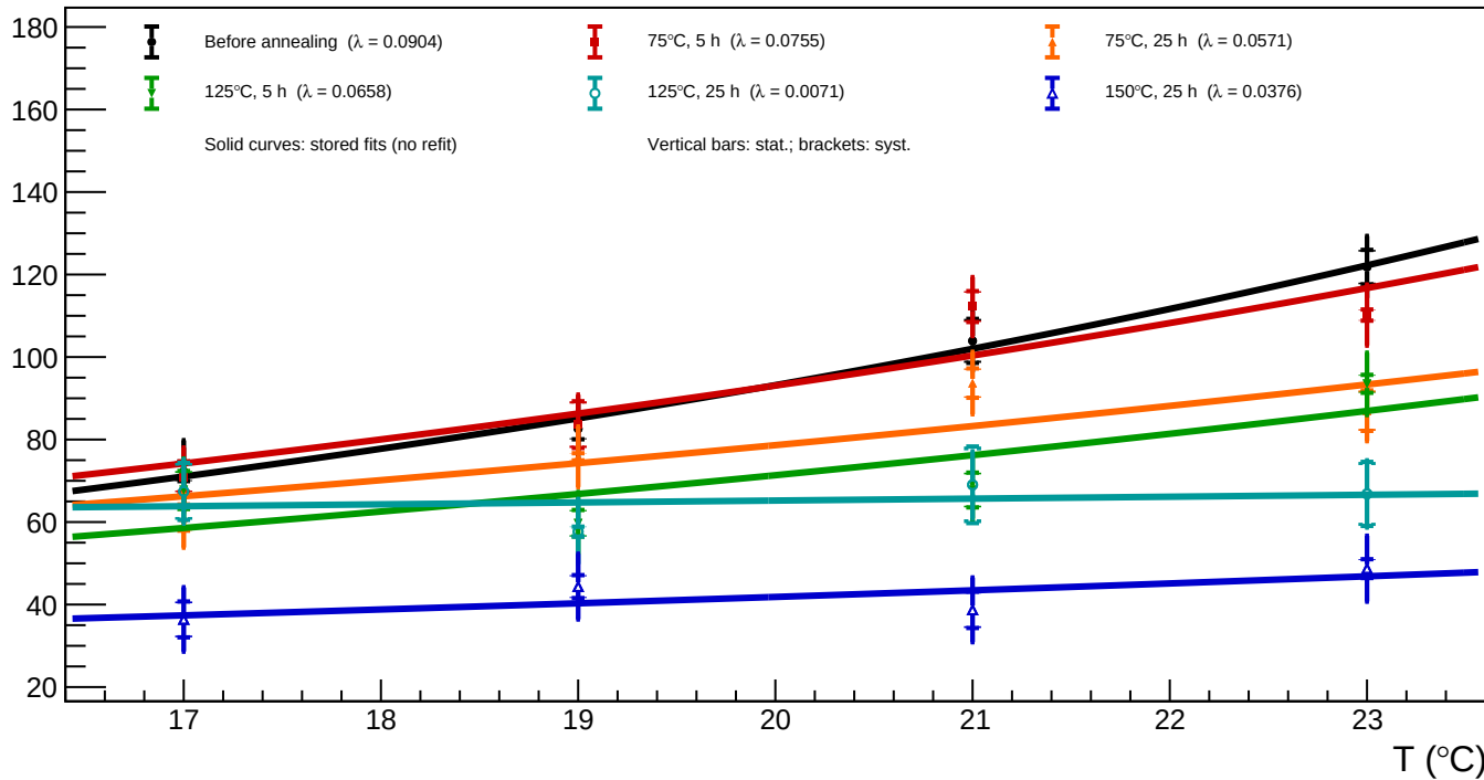
B1_v=3 - Spot 6 ( x = 233.20 , y = 473.06 ): luminosity vs temperature for all annealing phases
