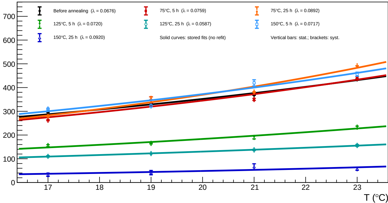
B1_v=3 - Spot 60 (x = 1832.49, y = 277.64): luminosity vs temperature for all annealing phases
