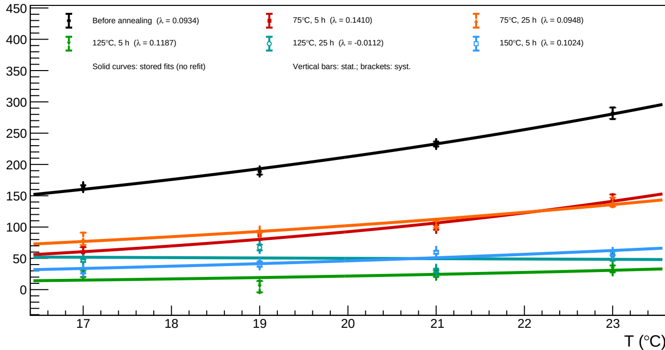
B1_v=3 - Spot 61 ( x = 1838.55 , y = 817.22 ): luminosity vs temperature for all annealing phases
