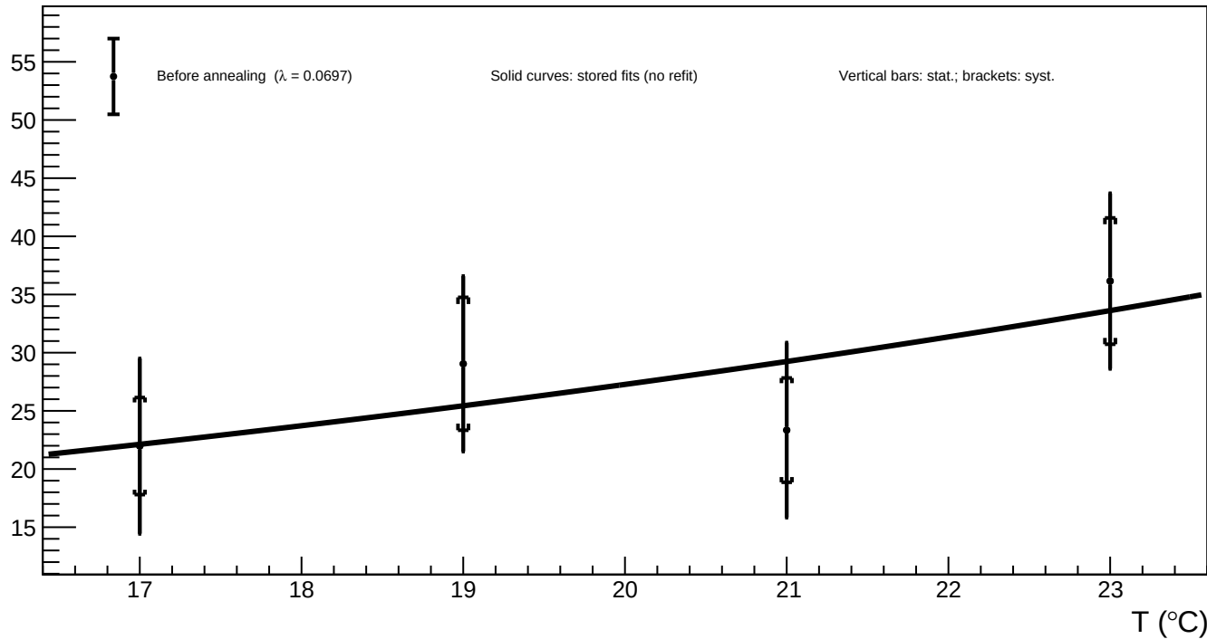
B1_v=3 - Spot 62 (x = 118.21, y = 98.99): luminosity vs temperature for all annealing phases
