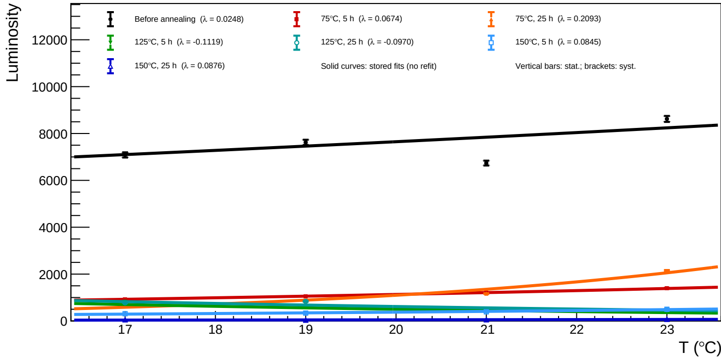
B1_v=3 - Spot 65 (x = 502.18, y = 522.13): luminosity vs temperature for all annealing phases
