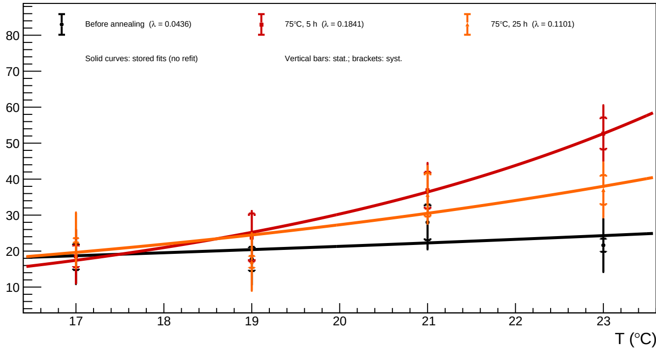
B1_v=3 - Spot 66 (x = 589.10, y = 234.50): luminosity vs temperature for all annealing phases
