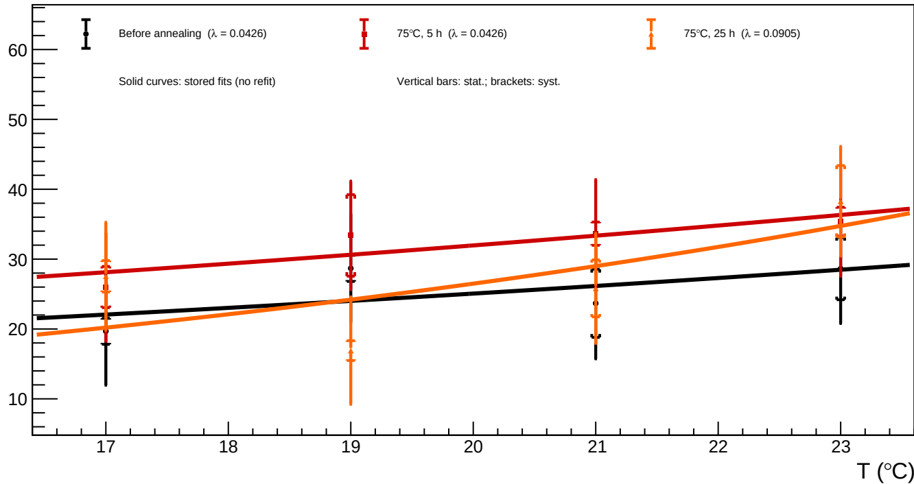
B1_v=3 - Spot 67 (x = 982.63, y = 929.17): luminosity vs temperature for all annealing phases
