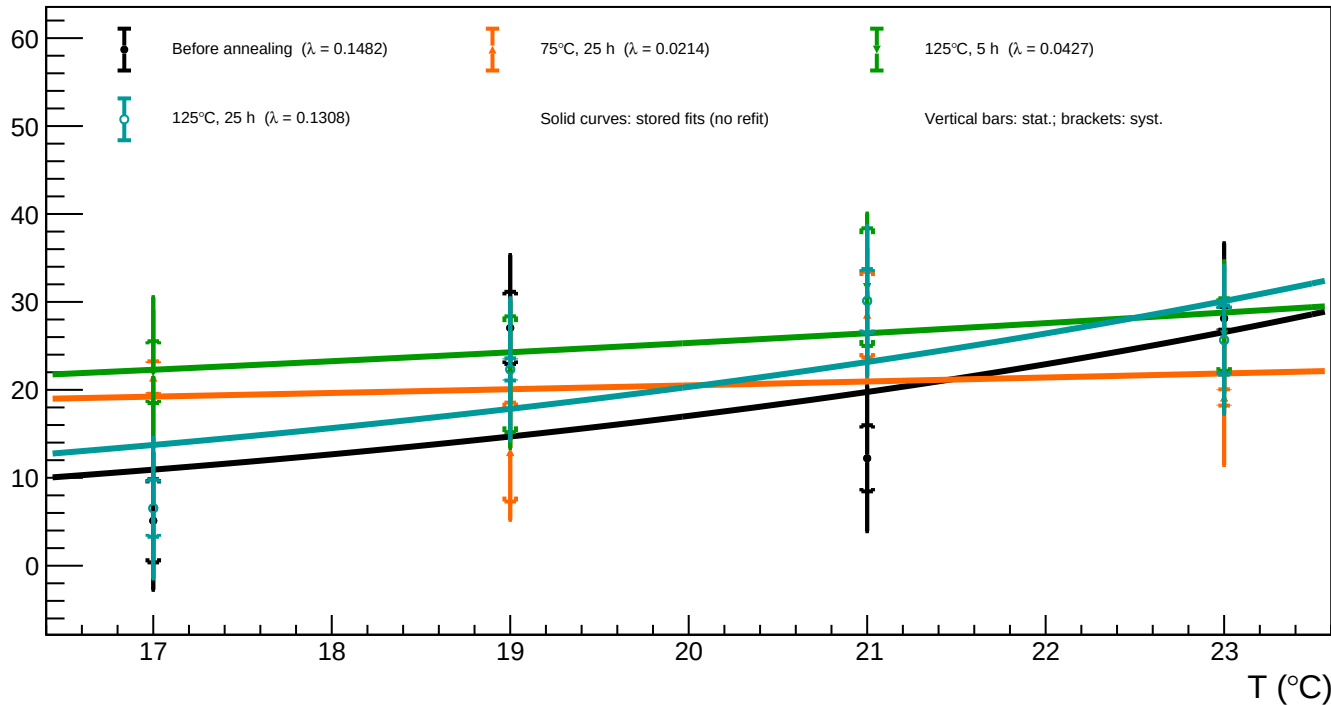
B1_v=3 - Spot 68 (x = 1200.84, y = 203.86): luminosity vs temperature for all annealing phases
