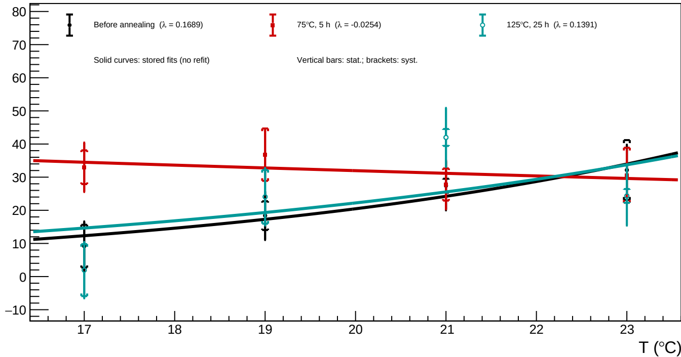
B1_v=3 - Spot 7 ( x = 276.65 , y = 942.02 ): luminosity vs temperature for all annealing phases
