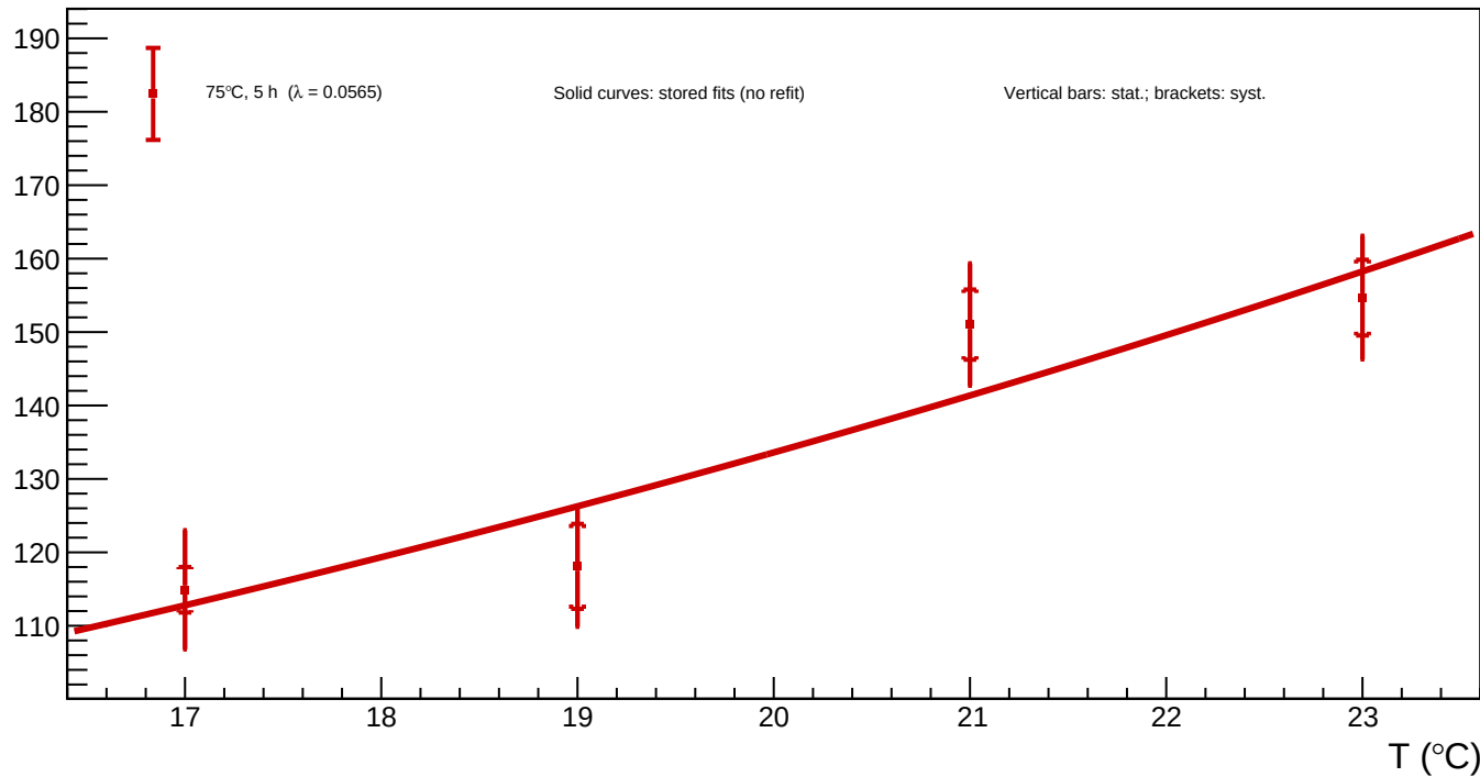
B1_v=3 - Spot 71 ( x = 150.27 , y = 226.61 ): luminosity vs temperature for all annealing phases
