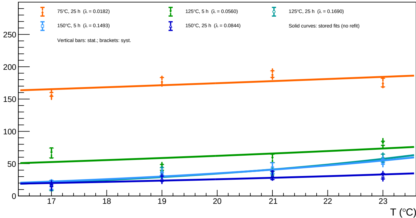
B1_v=3 - Spot 74 (x = 792.39, y = 461.11): luminosity vs temperature for all annealing phases
