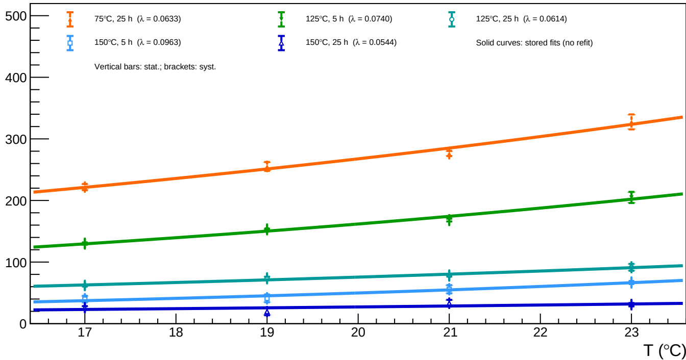
B1_v=3 - Spot 78 ( x = 1530.43 , y = 489.10 ): luminosity vs temperature for all annealing phases
