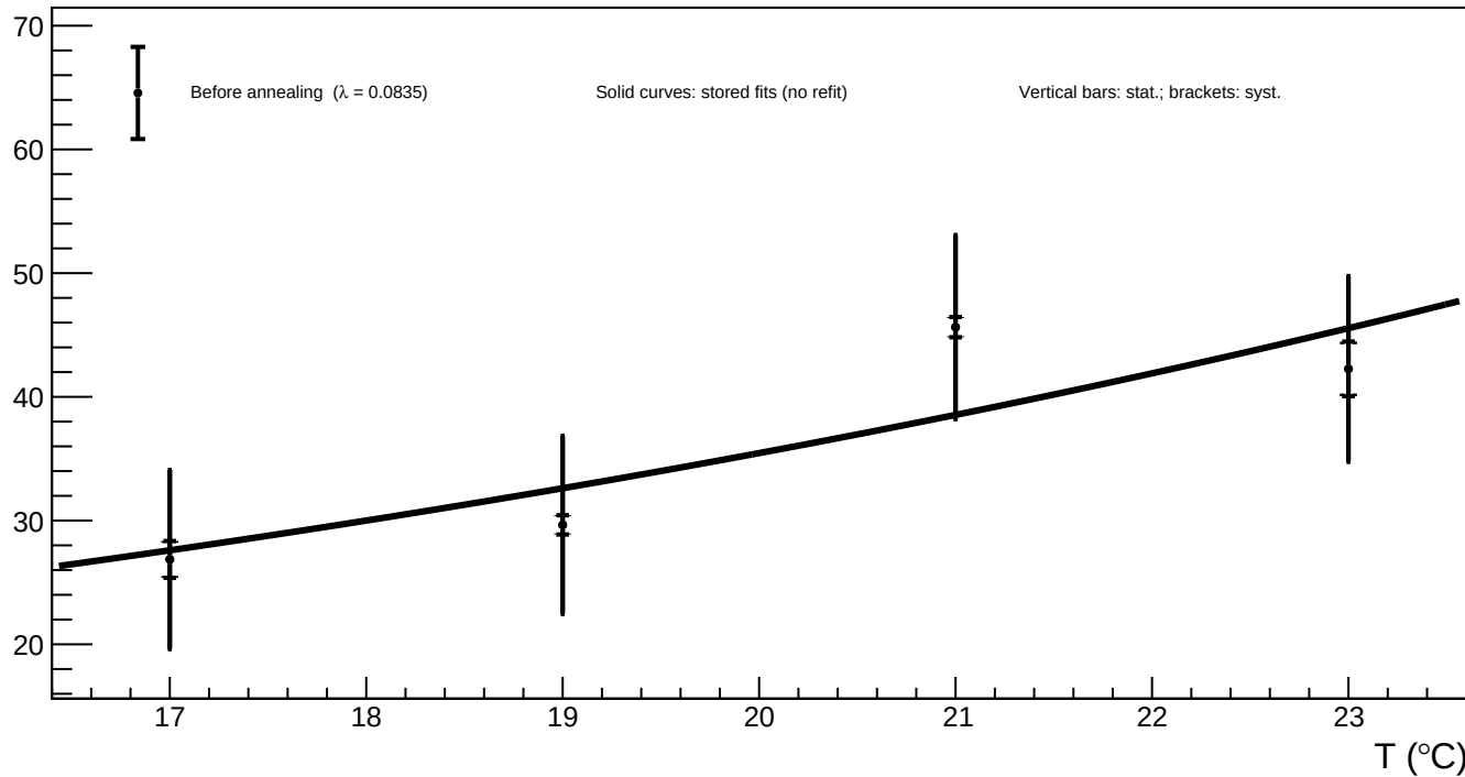
B1_v=3 - Spot 8 ( x = 287.60 , y = 753.98 ): luminosity vs temperature for all annealing phases
