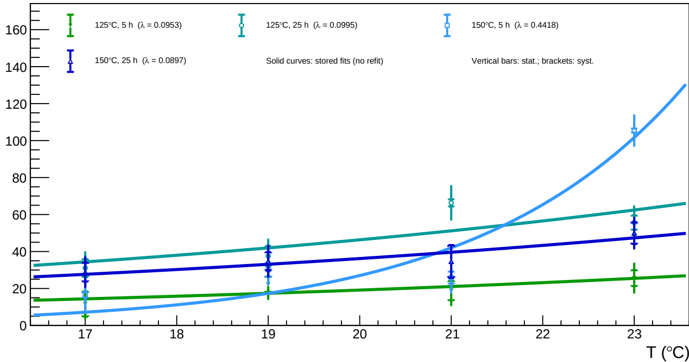
B1_v=3 - Spot 83 ( x = 1464.37 , y = 152.01 ): luminosity vs temperature for all annealing phases
