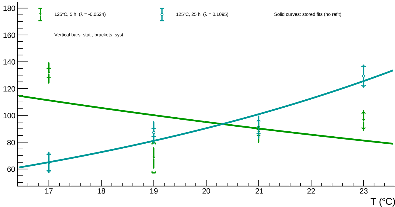
B1_v=3 - Spot 84 (x = 1744.34, y = 665.24): luminosity vs temperature for all annealing phases
