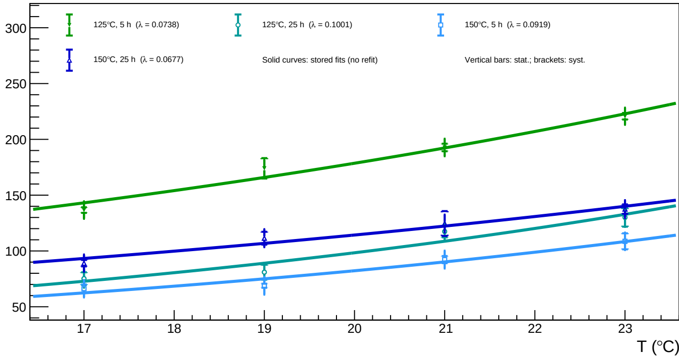
B1_v=3 - Spot 85 (x = 195.41, y = 133.55): luminosity vs temperature for all annealing phases
