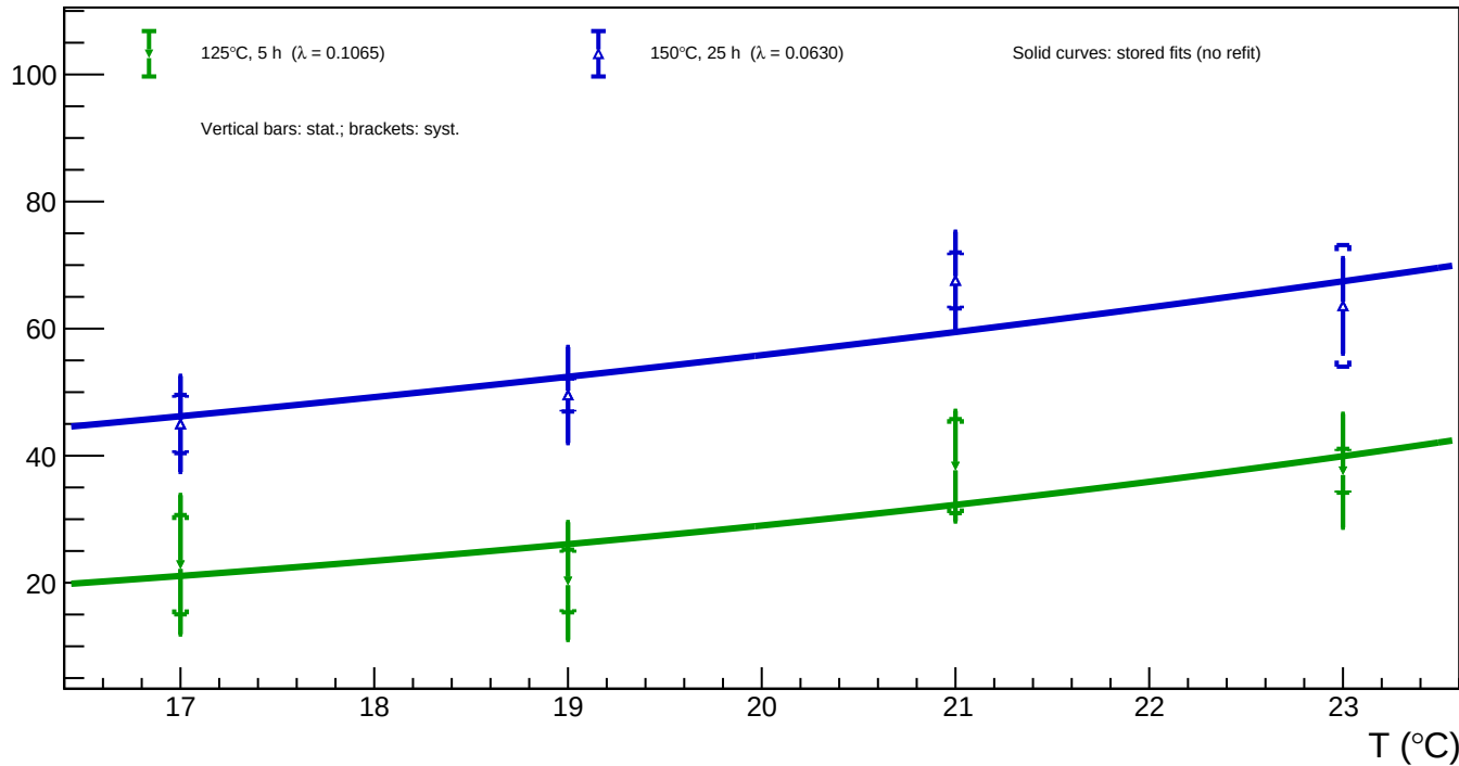
B1_v=3 - Spot 88 ( x = 370.42 , y = 1002.26 ): luminosity vs temperature for all annealing phases
