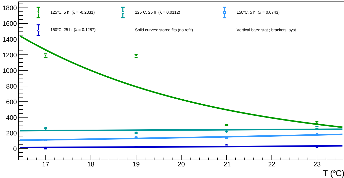
B1_v=3 - Spot 89 (x = 562.34, y = 287.07): luminosity vs temperature for all annealing phases
