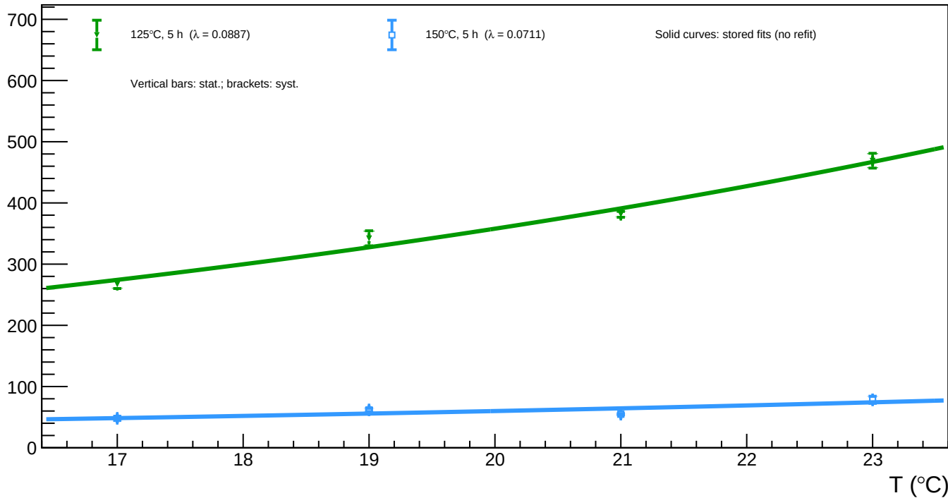
B1_v=3 - Spot 90 (x = 745.33, y = 904.37): luminosity vs temperature for all annealing phases
