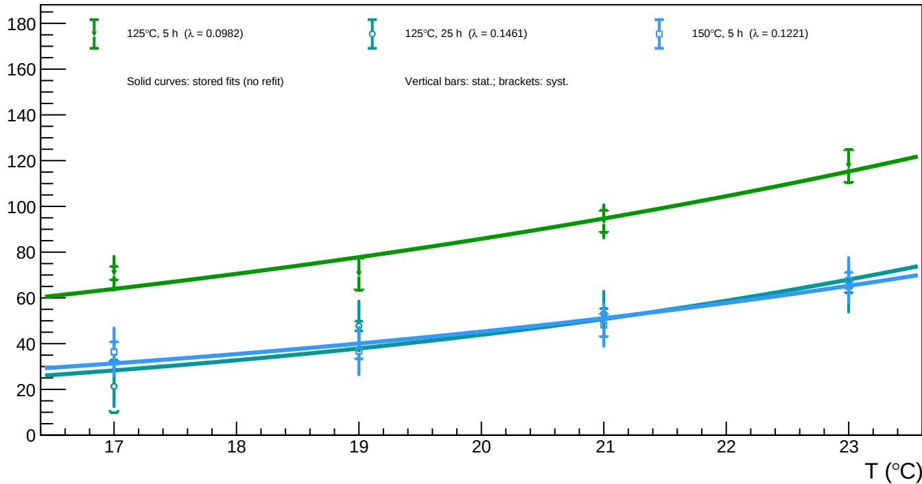
B1_v=3 - Spot 92 ( x = 1094.12 , y = 323.18 ): luminosity vs temperature for all annealing phases
