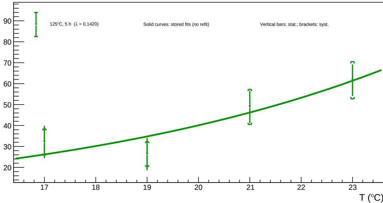
B1_v=3 - Spot 96 (x = 747.79, y = 86.96): luminosity vs temperature for all annealing phases
