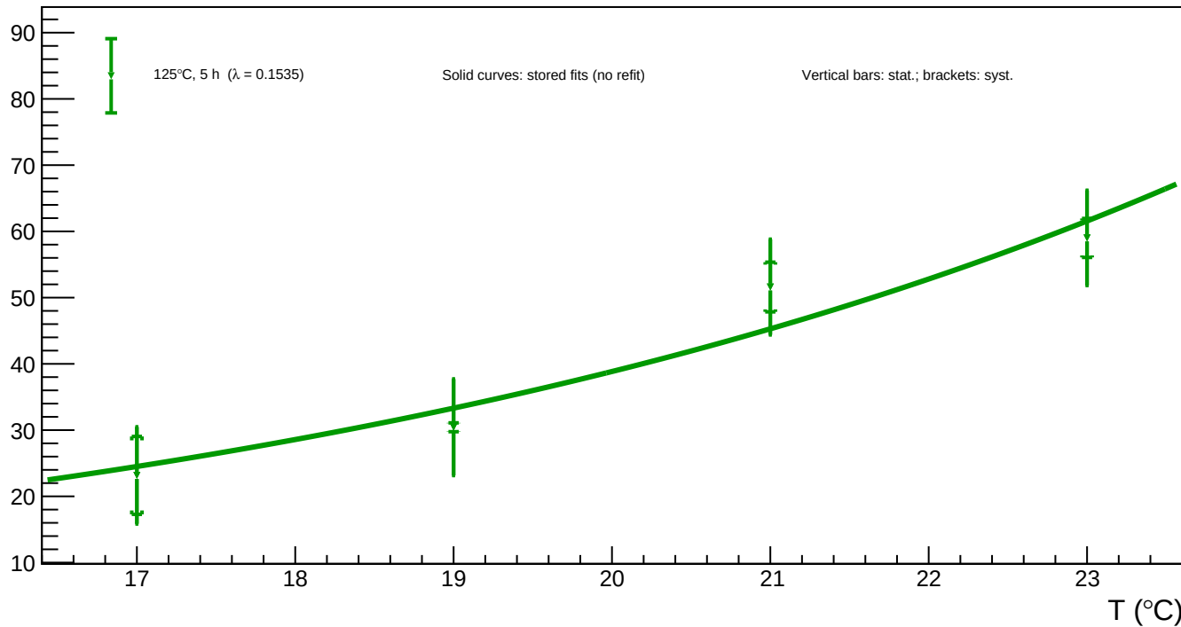
B1_v=3 - Spot 97 (x = 810.92, y = 735.32): luminosity vs temperature for all annealing phases
