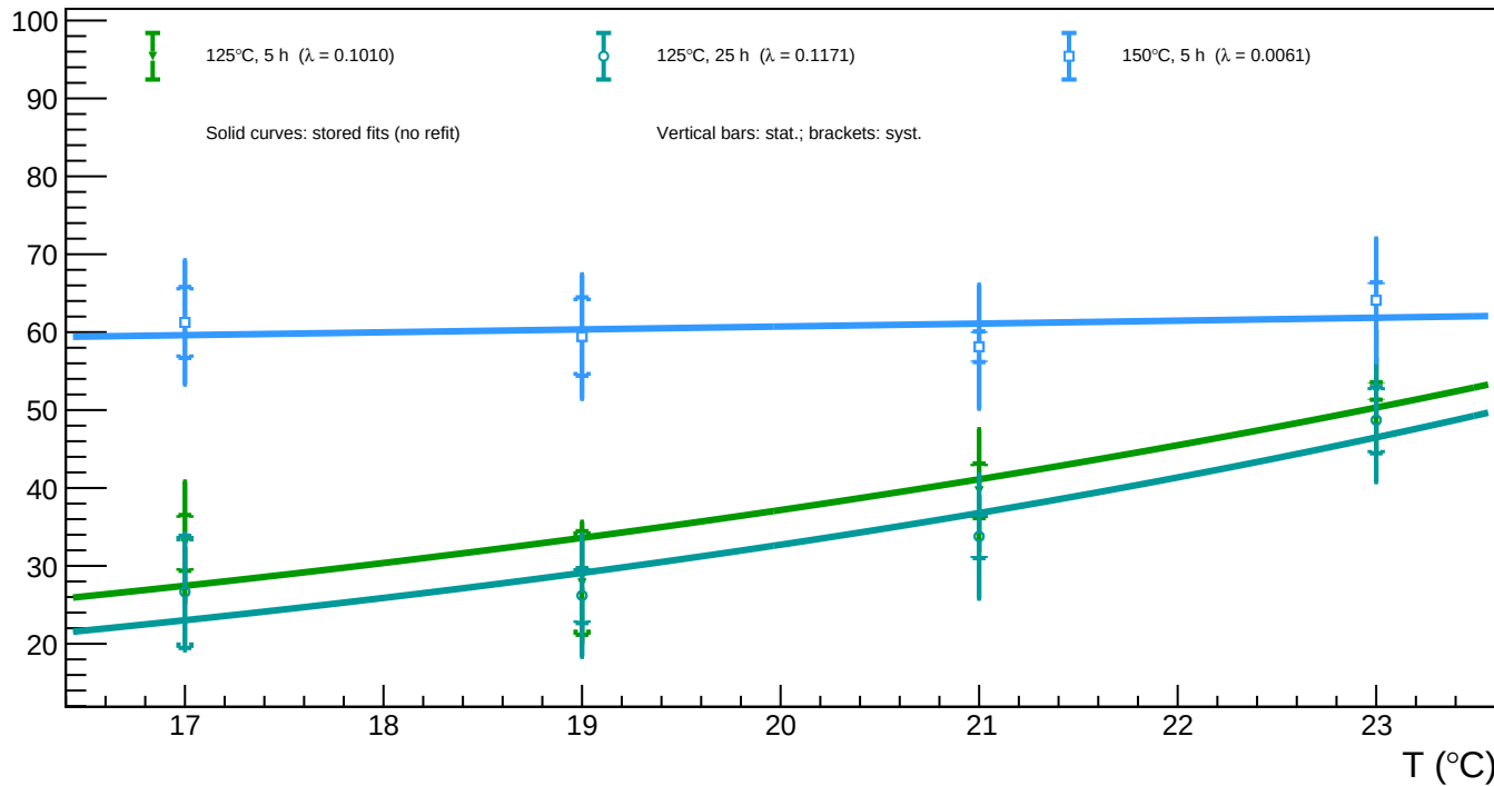
B1_v=3 - Spot 98 (x = 929.94, y = 206.68): luminosity vs temperature for all annealing phases
