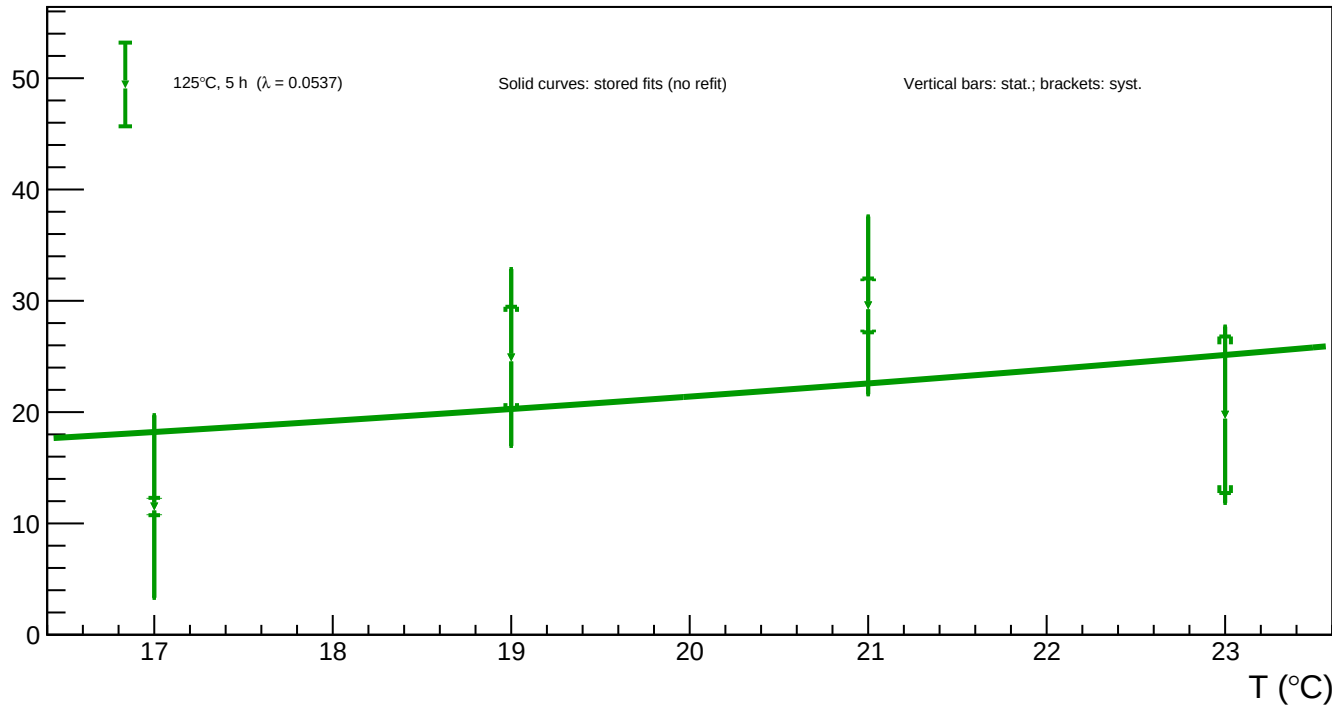
B1_v=3 - Spot 99 (x = 1453.59, y = 497.59): luminosity vs temperature for all annealing phases
