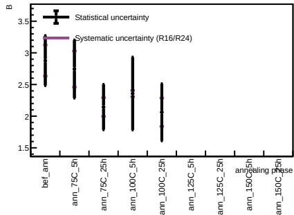
Sensor A1, T = 20 C - Spot 43
