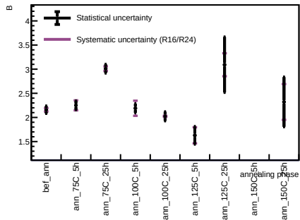
Sensor A1, T = 20 C - Spot 46
