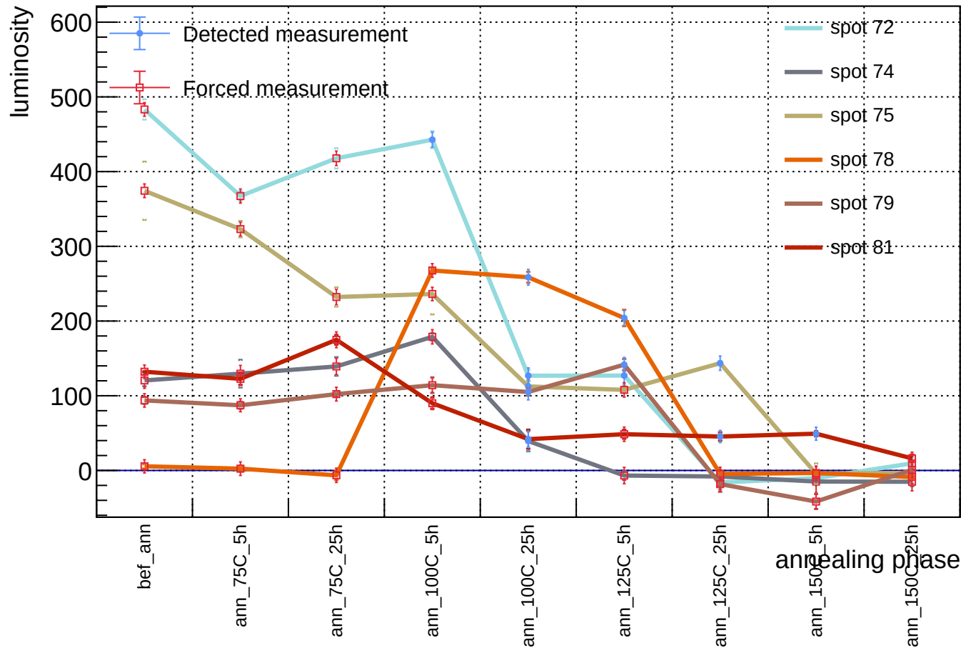
Sensor A1, T = 20\text{ C} , v_{\text{over}} = 7\text{ V} - luminosity vs phase - order 10^2
