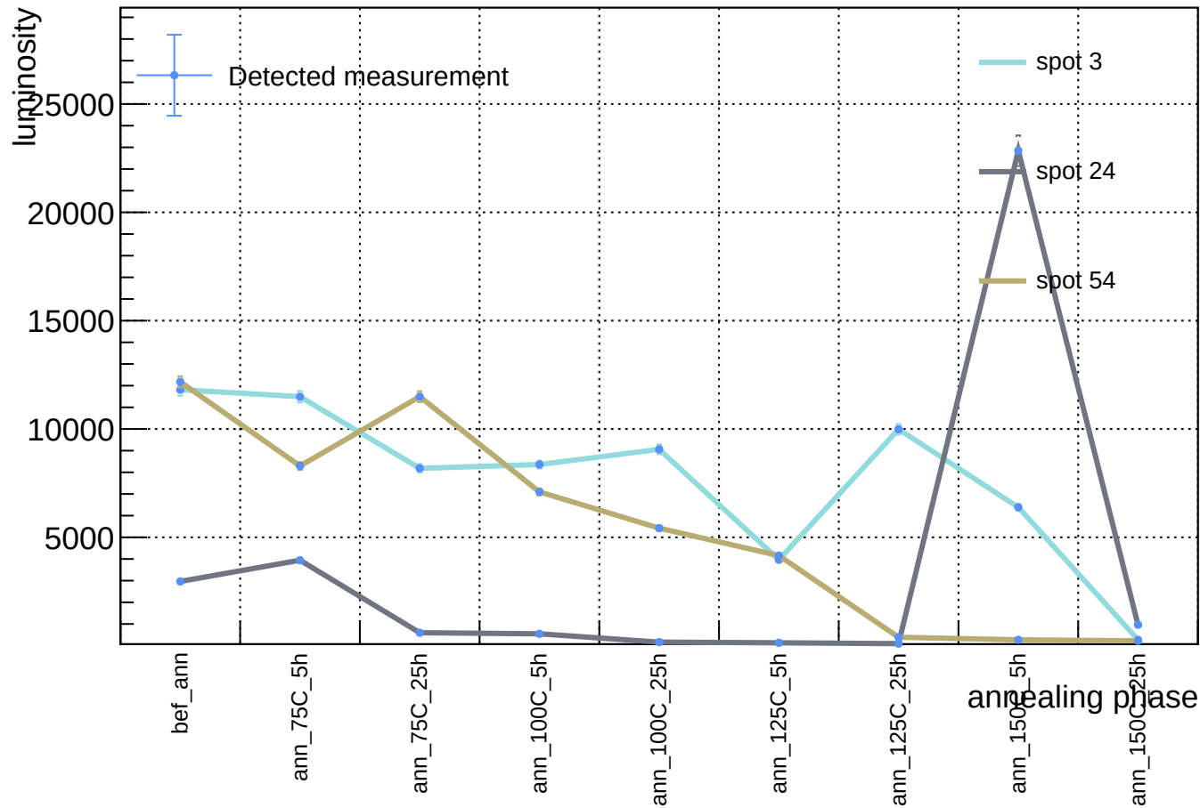
Sensor A1, T = 20\text{ C} , v_{\text{over}} = 7\text{ V} - luminosity vs phase - order 10^4
