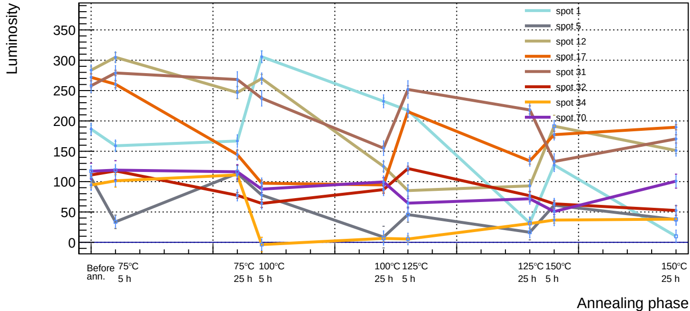
Sensor A1, T = 20\text{ }^{\circ}\text{C} , v_{\text{over}} = 7\text{ V} - Decreasing fluctuating, L < 800
