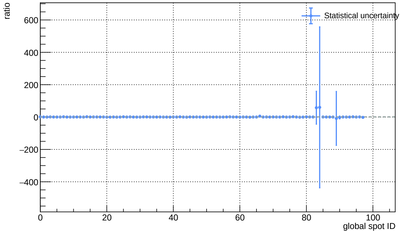
Sensor A1, T = 20 C - L(\text{ann\_125C\_25h}) / L(\text{before\_annealing})
