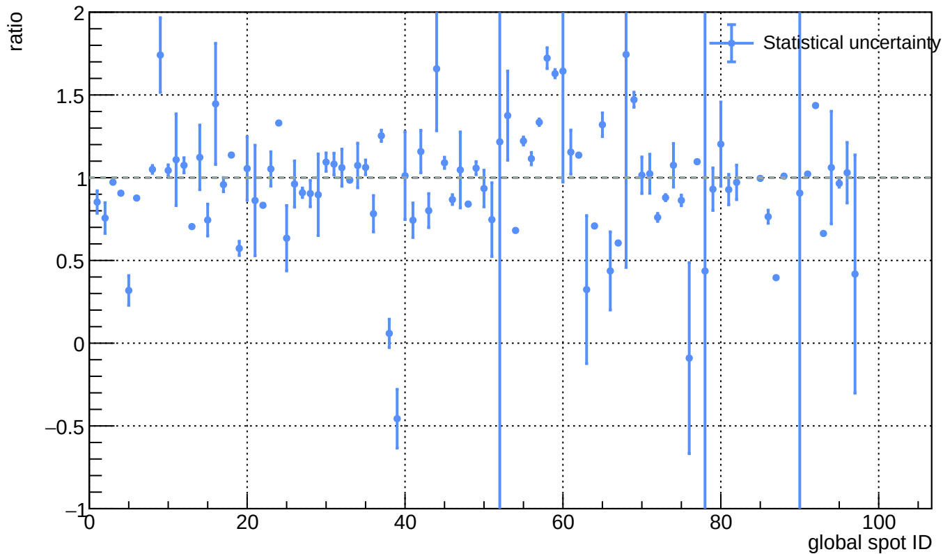
Sensor A1, T = 20 C - L(ann_75C_5h) / L(before_annealing)
