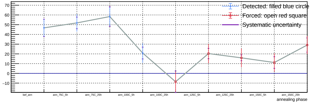
Sensor A1, T = 20\text{ C} , v_{\text{over}} = 7\text{ V} - Spot 11: luminosity vs phase
