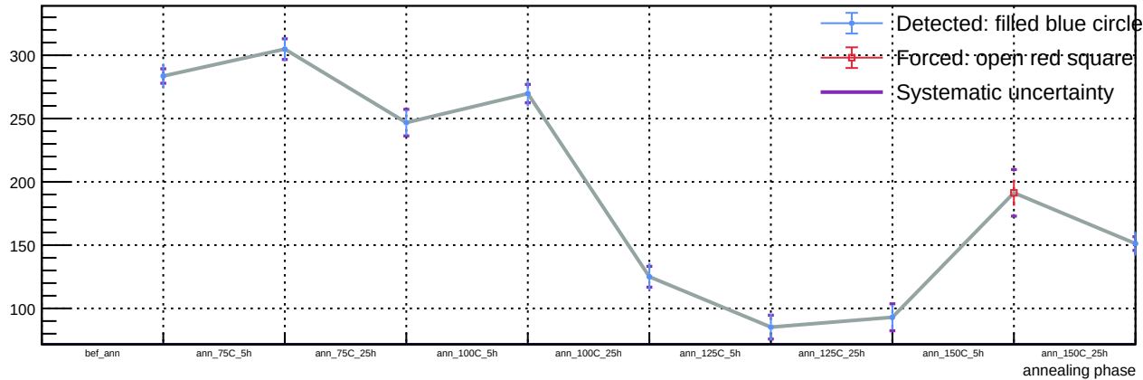
Sensor A1, T = 20\text{ C} , v_{\text{over}} = 7\text{ V} - Spot 12: luminosity vs phase
