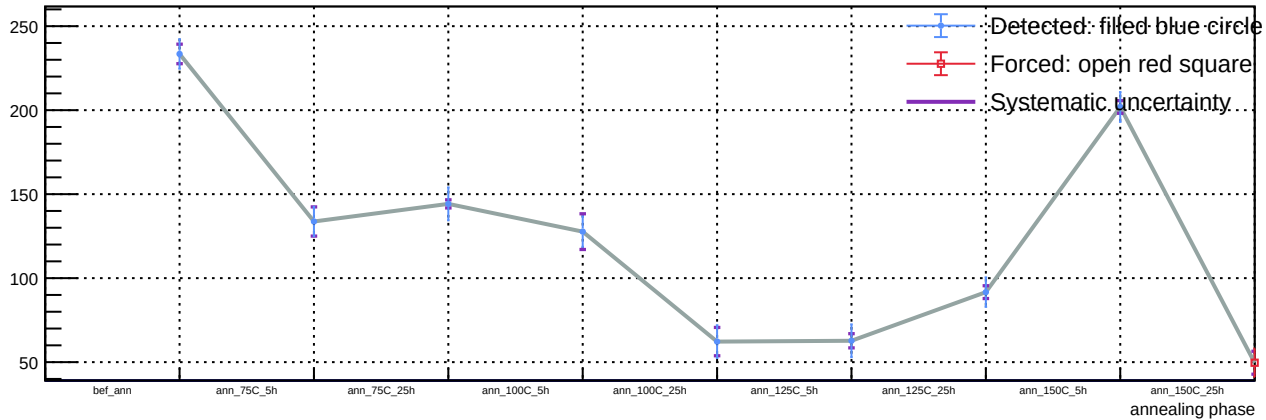
Sensor A1, T = 20\text{ C} , v_{\text{over}} = 7\text{ V} - Spot 19: luminosity vs phase
