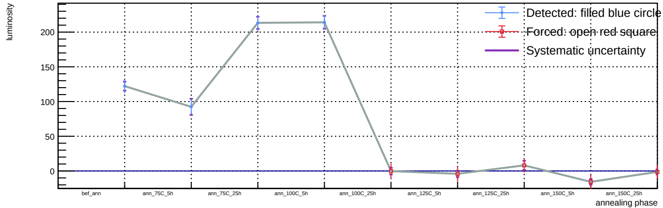
Sensor A1, T = 20\text{ C} , v_{\text{over}} = 7\text{ V} - Spot 2: luminosity vs phase
