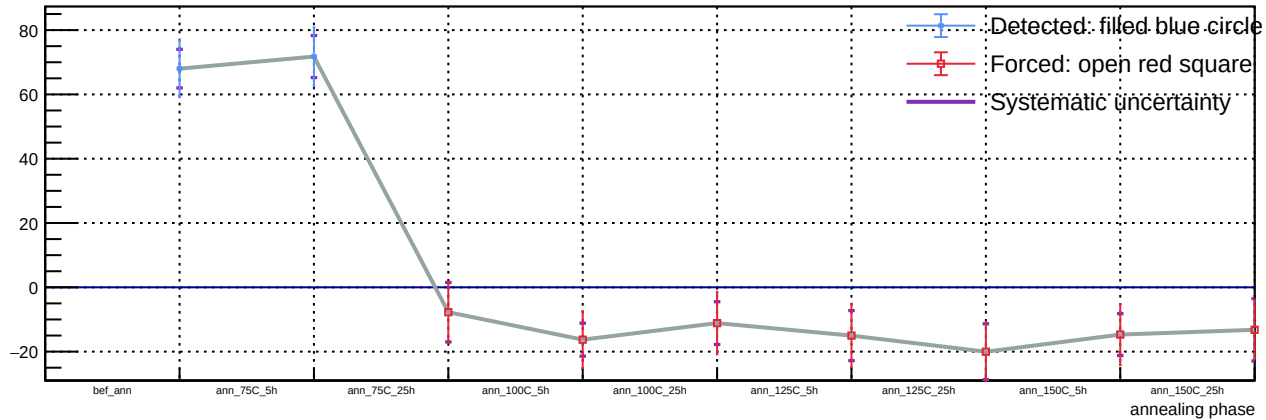
Sensor A1, T = 20\text{ C} , v_{\text{over}} = 7\text{ V} - Spot 20: luminosity vs phase
