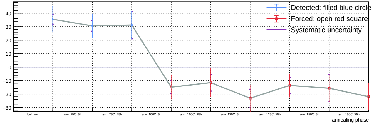
Sensor A1, T = 20\text{ C} , v_{\text{over}} = 7\text{ V} - Spot 21: luminosity vs phase
