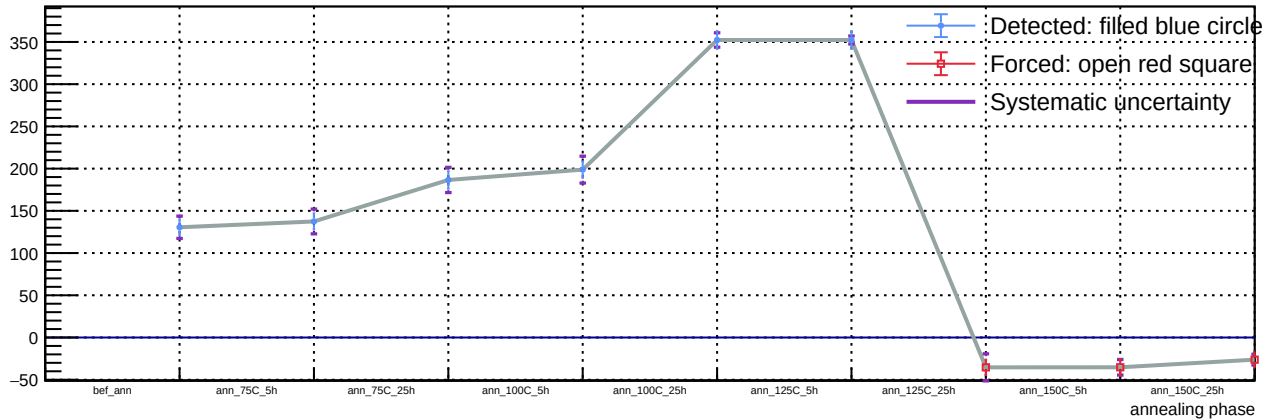
Sensor A1, T = 20\text{ C} , v_{\text{over}} = 7\text{ V} - Spot 23: luminosity vs phase
