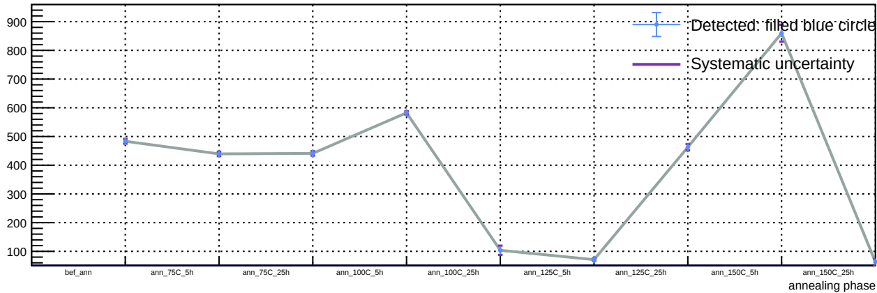
Sensor A1, T = 20\text{ C} , v_{\text{over}} = 7\text{ V} - Spot 27: luminosity vs phase
