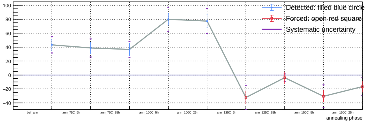
Sensor A1, T = 20\text{ C} , v_{\text{over}} = 7\text{ V} - Spot 29: luminosity vs phase
