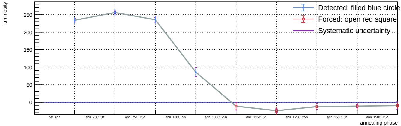
Sensor A1, T = 20\text{ C} , v_{\text{over}} = 7\text{ V} - Spot 30: luminosity vs phase
