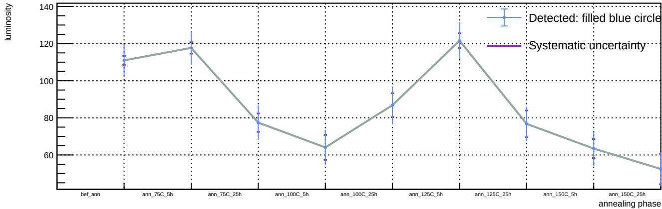
Sensor A1, T = 20\text{ C} , v_{\text{over}} = 7\text{ V} - Spot 32: luminosity vs phase
