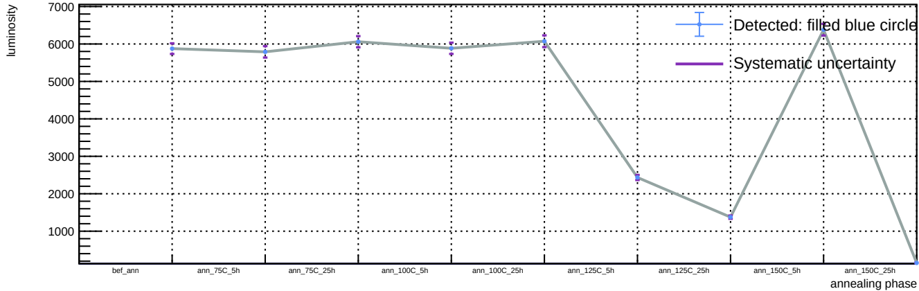
Sensor A1, T = 20\text{ C} , v_{\text{over}} = 7\text{ V} - Spot 33: luminosity vs phase
