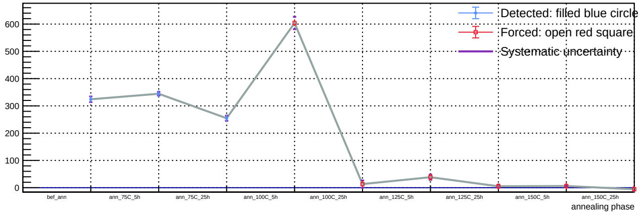
Sensor A1, T = 20\text{ C} , v_{\text{over}} = 7\text{ V} - Spot 35: luminosity vs phase
