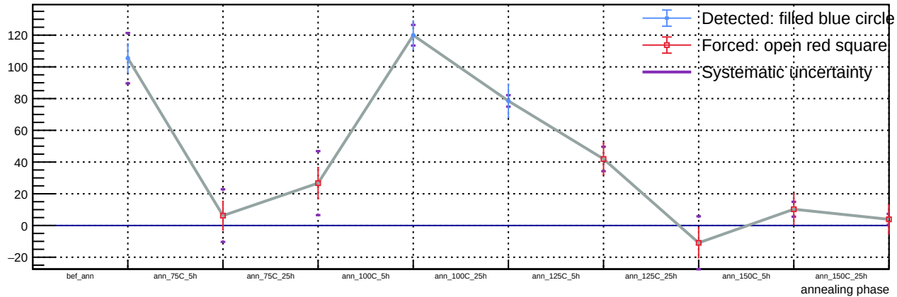
Sensor A1, T = 20\text{ C} , v_{\text{over}} = 7\text{ V} - Spot 38: luminosity vs phase
