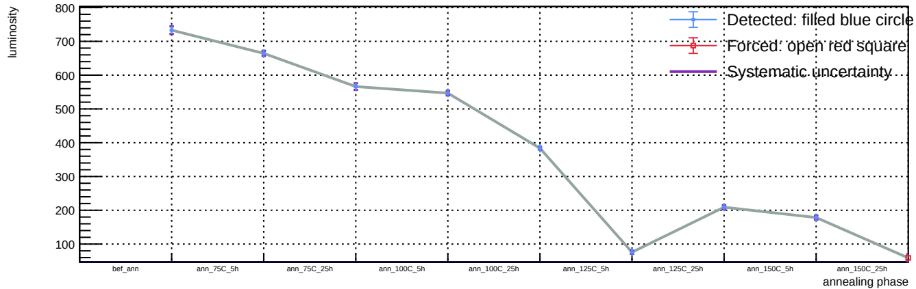
Sensor A1, T = 20\text{ C} , v_{\text{over}} = 7\text{ V} - Spot 4: luminosity vs phase
